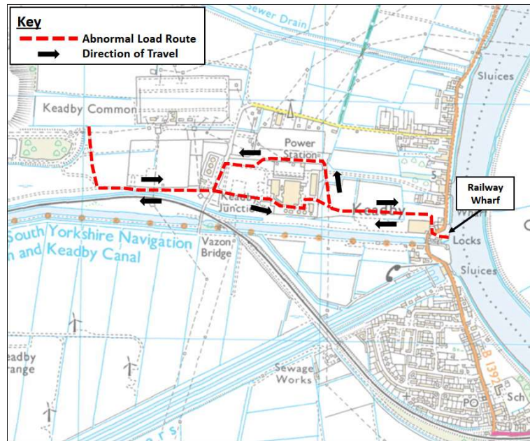
Figure 3: Updated Abnormal Indivisible Load Route via Waterborne Transport Offloading Area for Proposed Development
